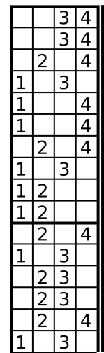
Double tabby v1 liftplan, with tabby
